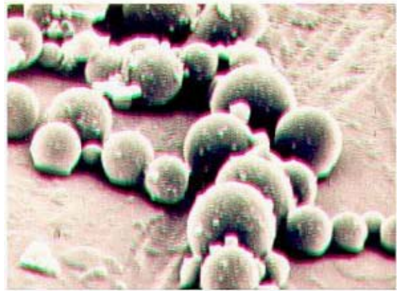
Coal Fly Ash
