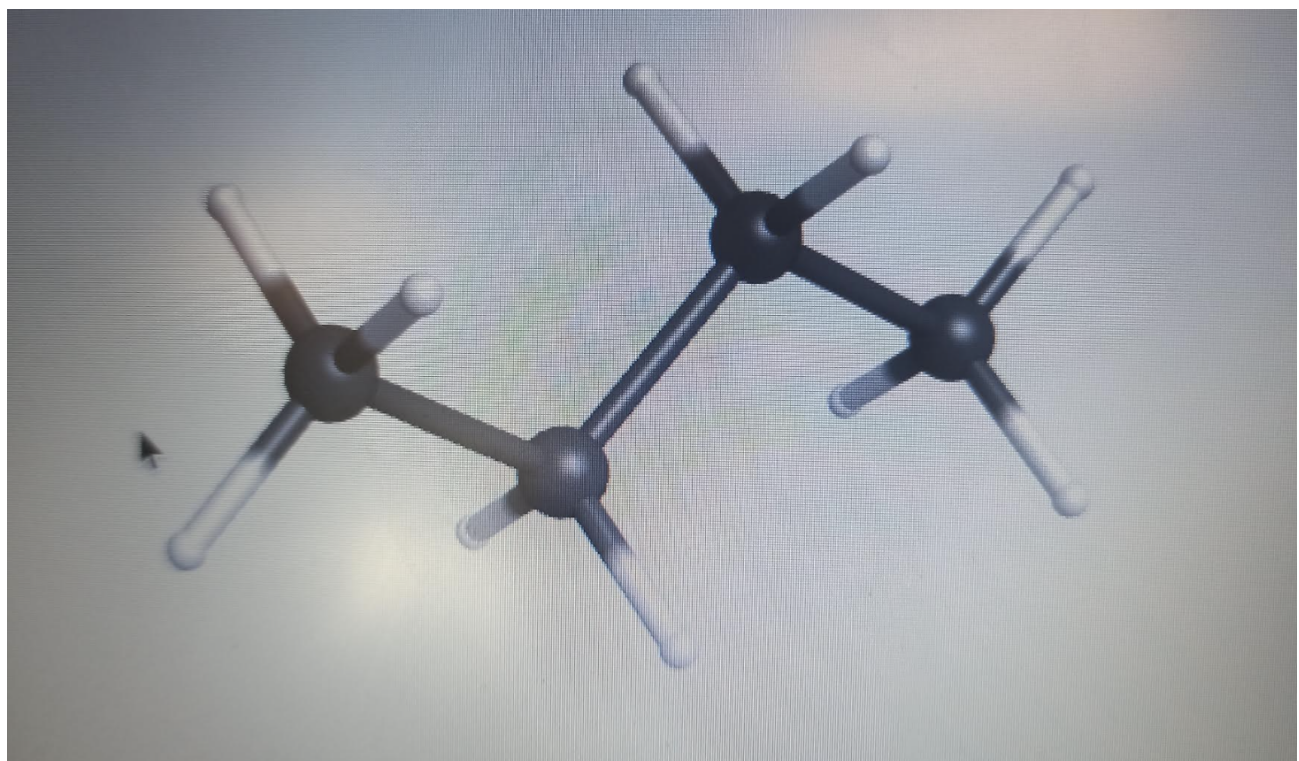
Butane (student model)
