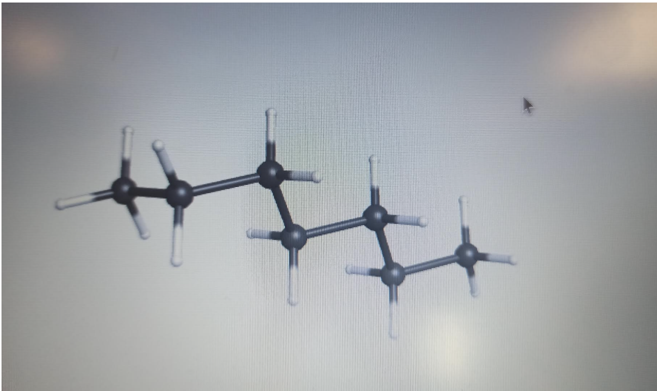
Heptane (student model)
