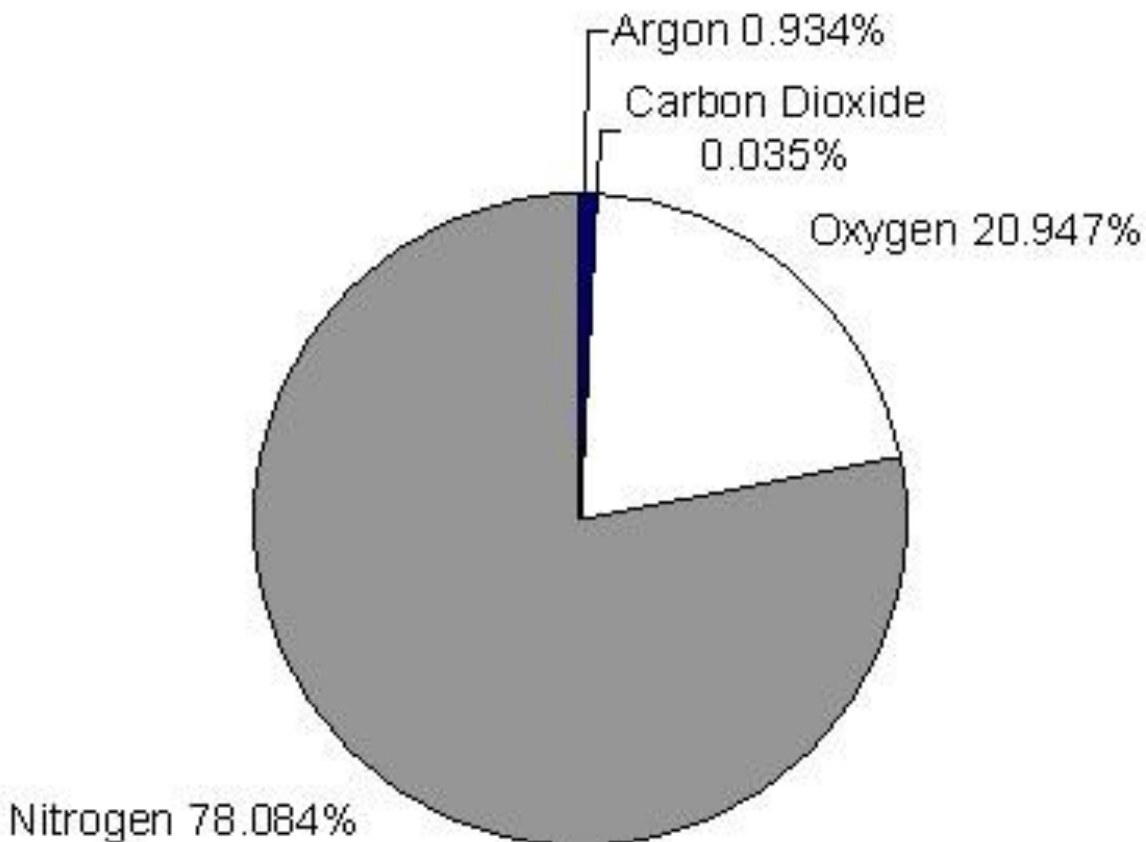
Gaseous Composition of Dry Air
