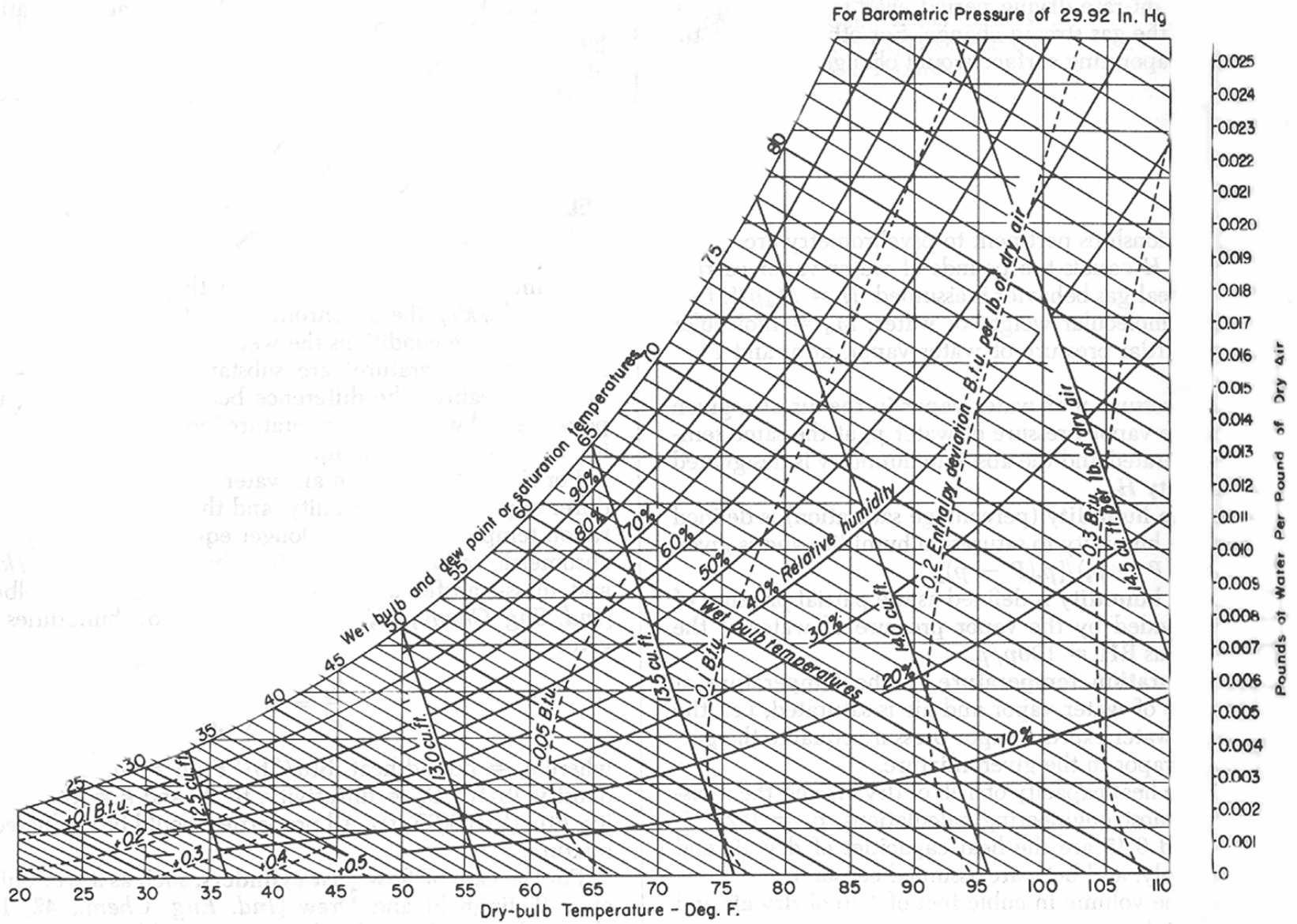
Air Pollution: Lesson 4, Dripping Wet or Dry as a Bone? Activity — Relative Humidity Graph Source: Perry, Robert H., Perry's Chemical Engineers' Handbook , Sixth Edition, Texas: McGraw-Hill, 1984, Figure 12-2 (Modified).
