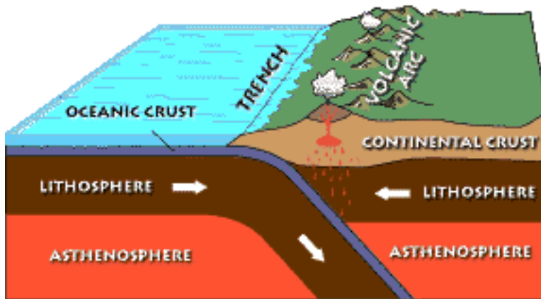
Oceanic vs. Continental Plate Convergence
