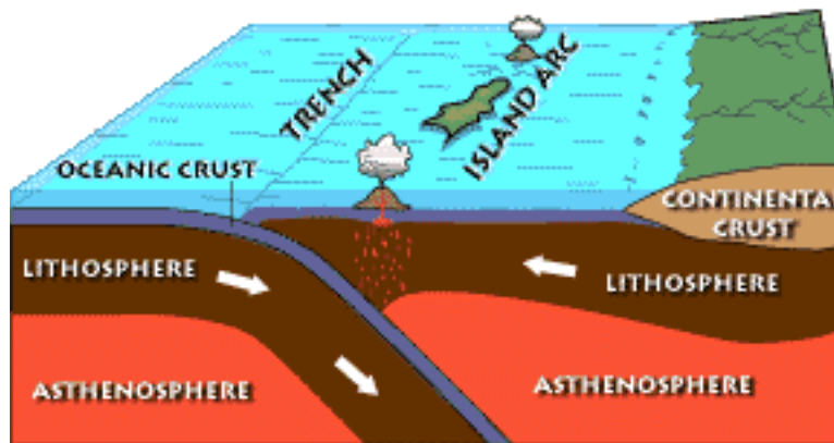
Oceanic vs. Oceanic Plate Convergence
