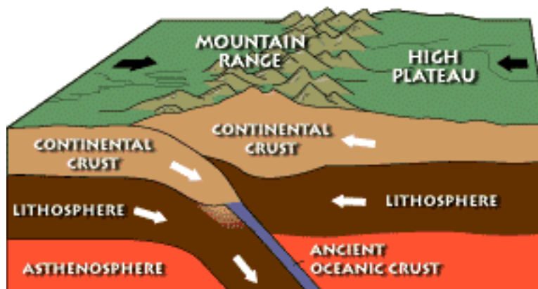
Continental vs. Continental Plate Convergence
