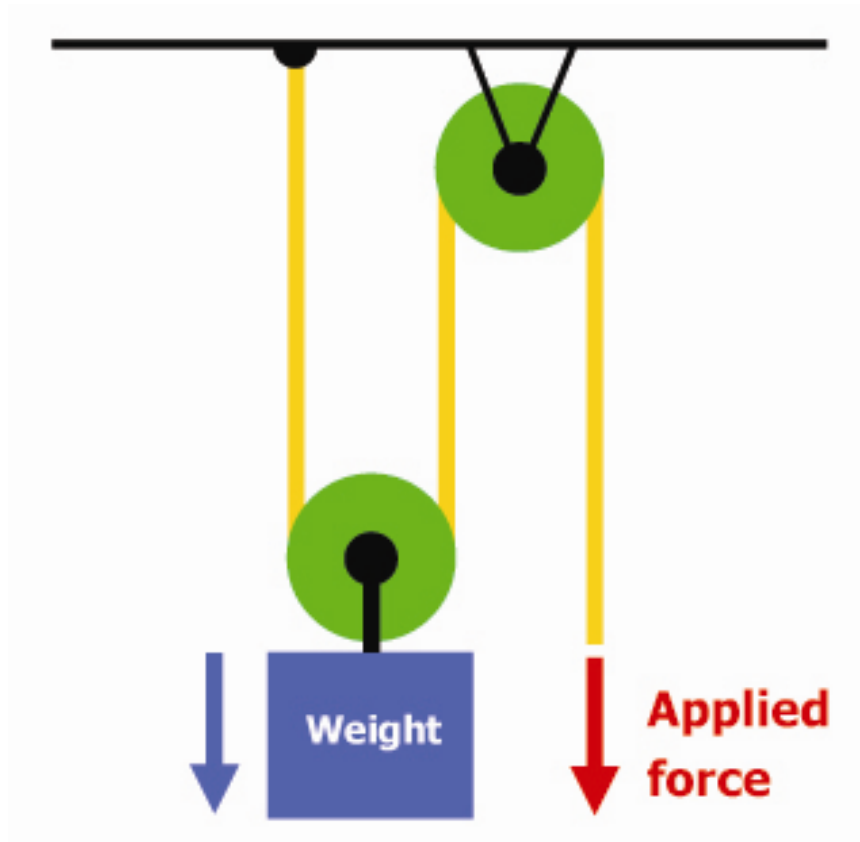
A two-pulley system with one movable pulley and one fixed pulley, and a mechanical advantage of two.
