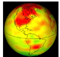
Global Warming 5
