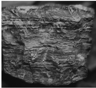
Coal 1
