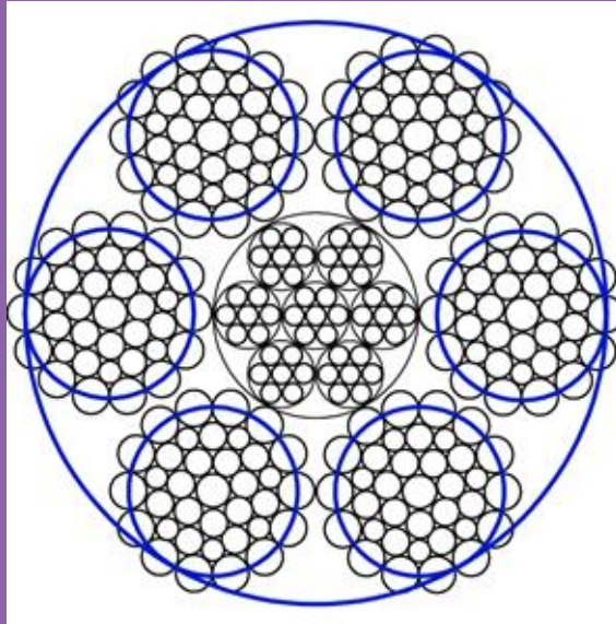
Figure 2: Cross-section of a steel cable (drawing)
